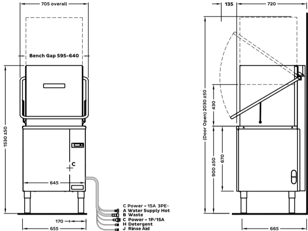
Bench detail
