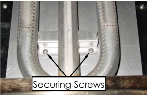
Main Burner - CR9 Model
